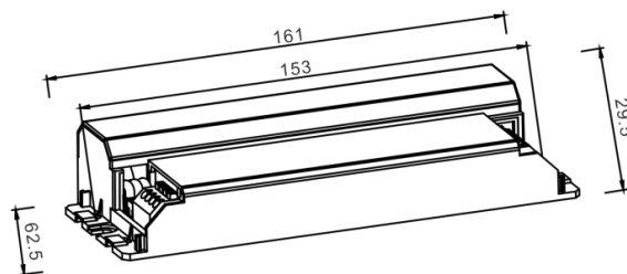
26650 battery built-in product size
