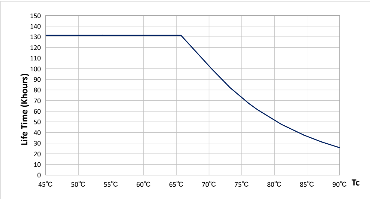
Lifetime Curve
