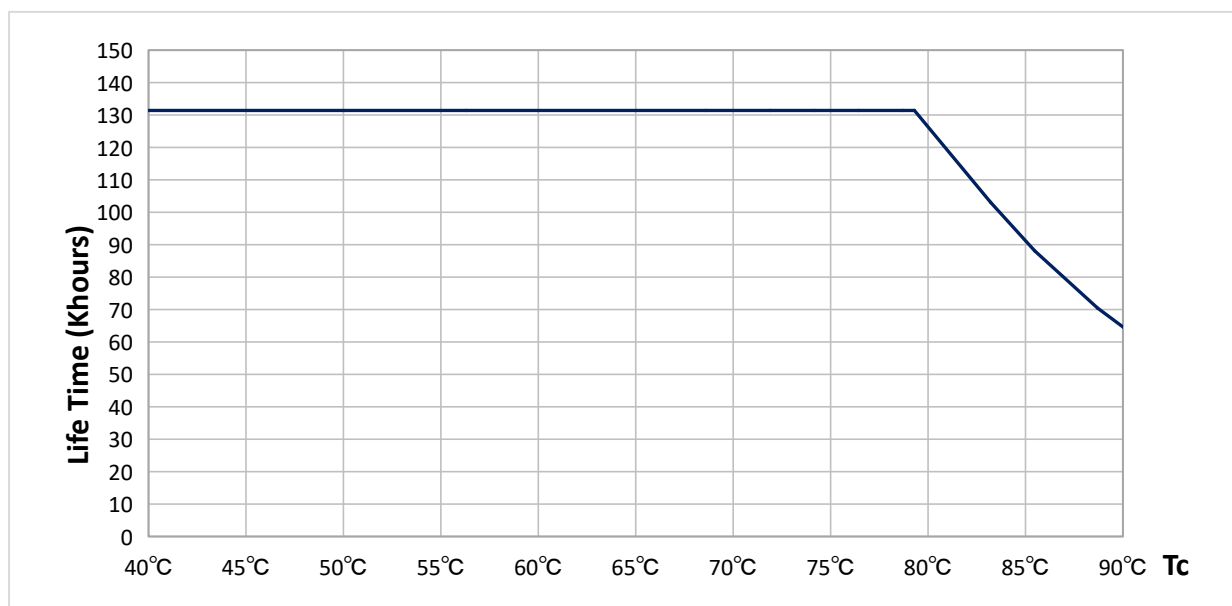
Lifetime Curve
