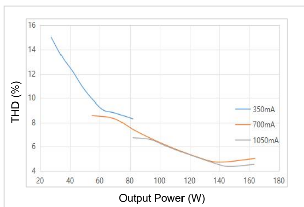
THD Curve
