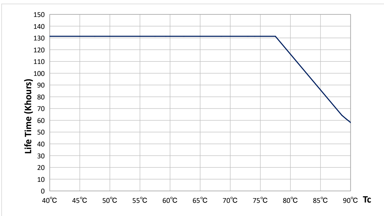
Lifetime Curve
