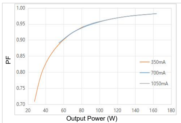
PF Curve
