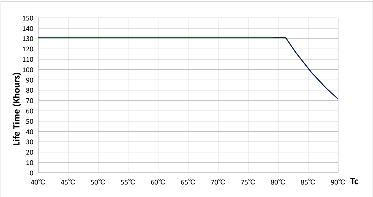
Lifetime Curve
