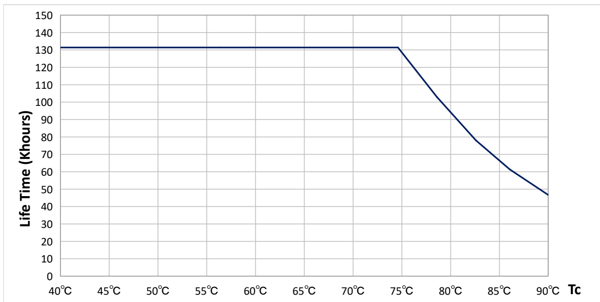
Lifetime Curve
