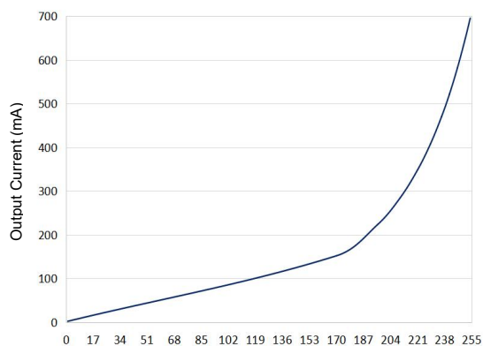
Logarithmic dimming
