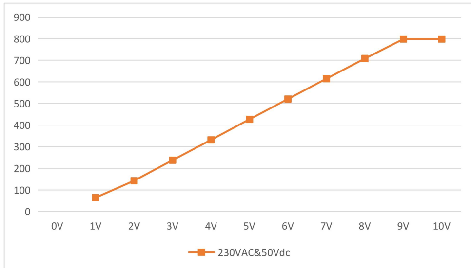
Dimming Curve
