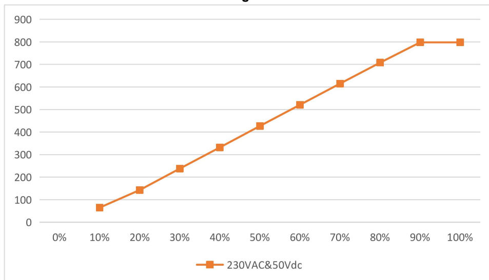
Dimming Curve
