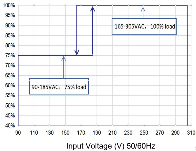
Load Derating Curve
