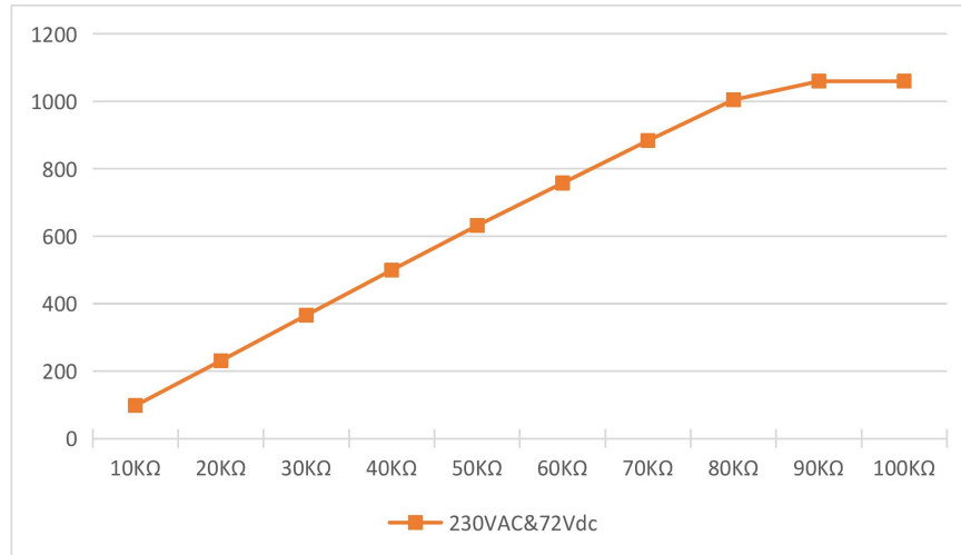
Dimming Curve
