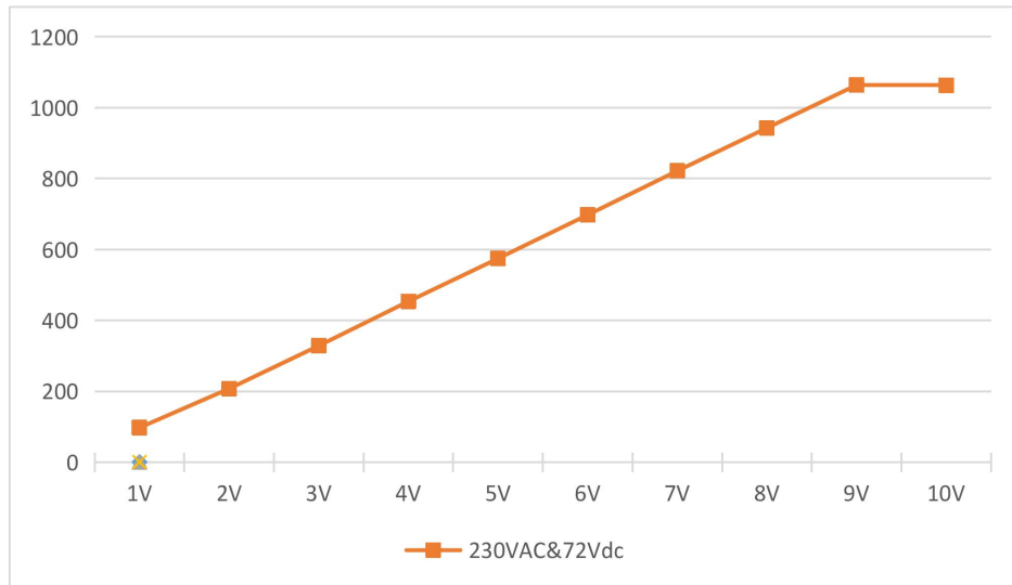
Dimming Curve
