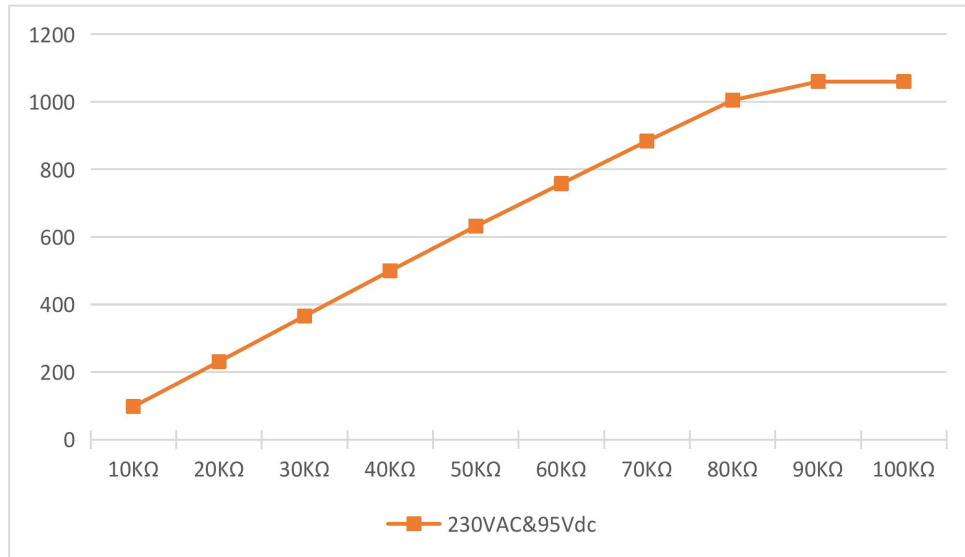
Dimming Curve
