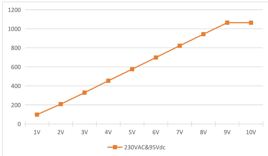
Dimming Curve
