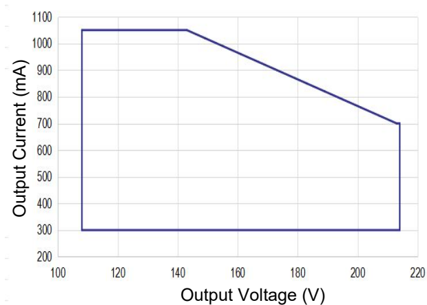
Operating Window
