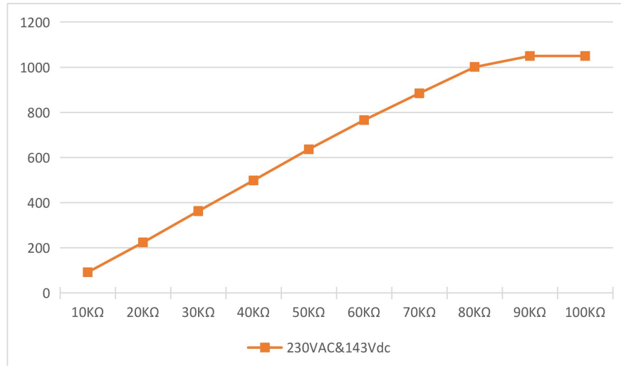
Dimming Curve
