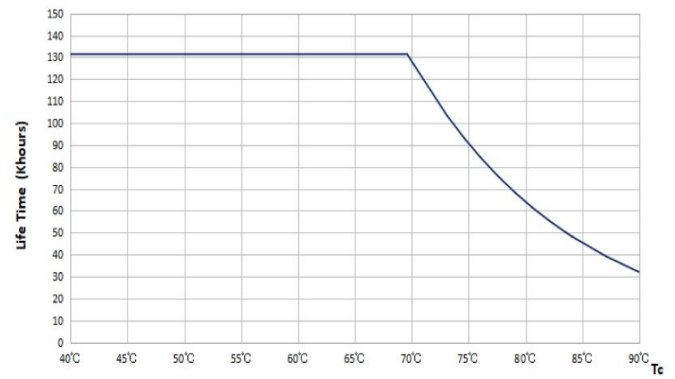
Lifespan
