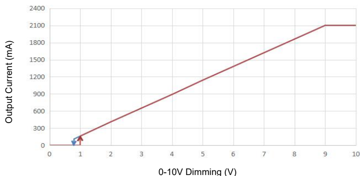
Dimming Curve
