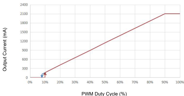
Dimming Curve
