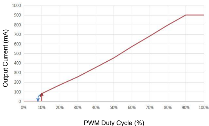
Dimming Curve
