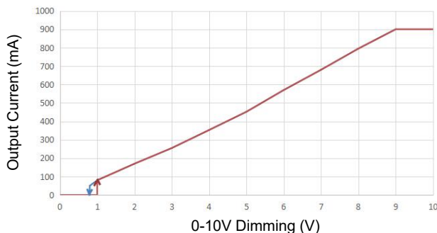
Dimming Curve
