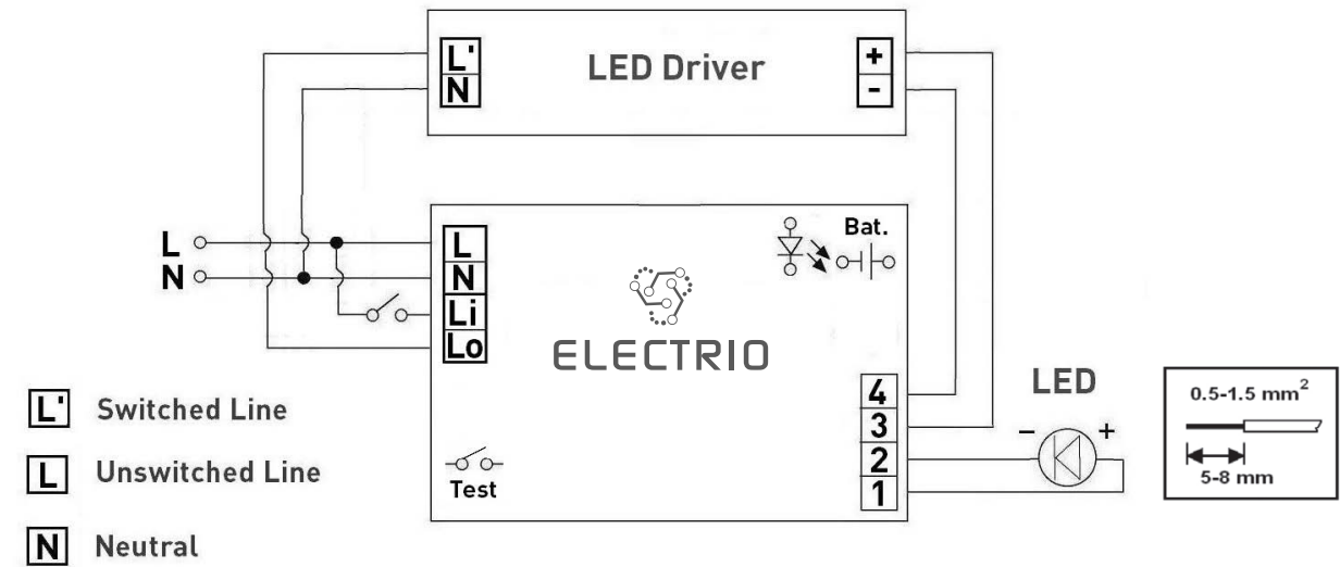
Wiring Diagram
